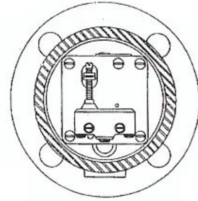
SECTION 13-13
